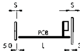
PCB: Circuito stampato (1,8 mm max) Printed circuit board (1,8 mm max)
